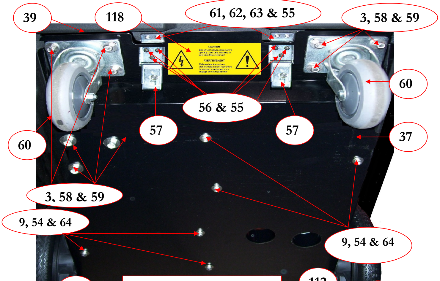
BOTTOM VIEW OF BASE
